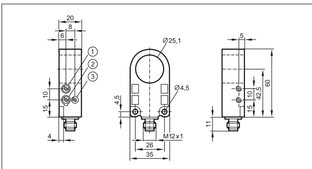
1: Sensitivity, 2: Output function, 3: Pulse stretching time
