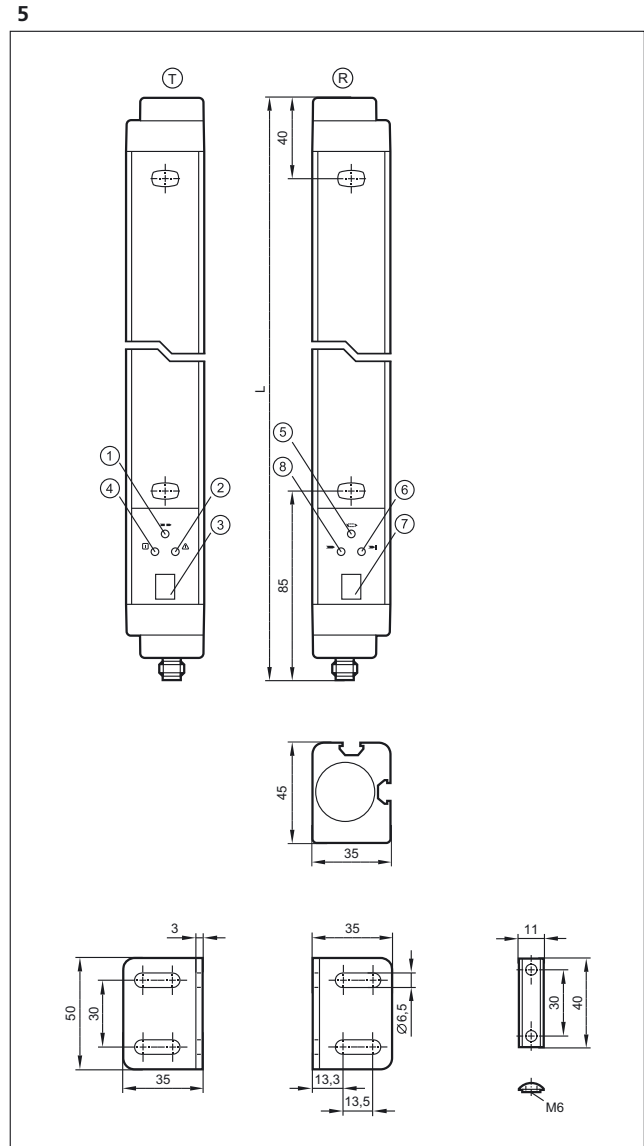
T: Transmitter, R: Receiver, 1: LED yellow, 2: LED red, 3: 7-segment LED display, 4: LED green, 5: LED yellow, 6: LED red, 7: 7-segment LCD display, 8: LED green
