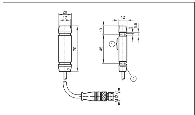
1: sensing face, 2: LED operating status
