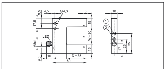
1: potentiometer sensitivity, 2: output function switch
