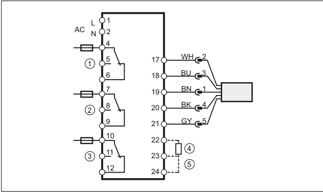
1: Flow monitoring, 2: Wire break monitoring, 3: Temperature monitoring, 4: Power-on delay time, 5: Selection liquid / gas
