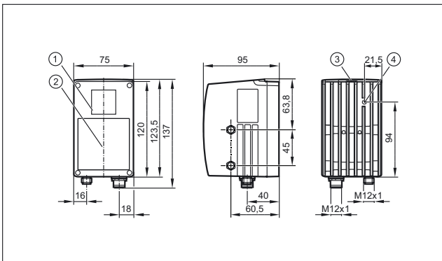
1: lens, 2: Illumination unit, 3: Display / buttons / LEDs, 4: Focus adjustment screw
