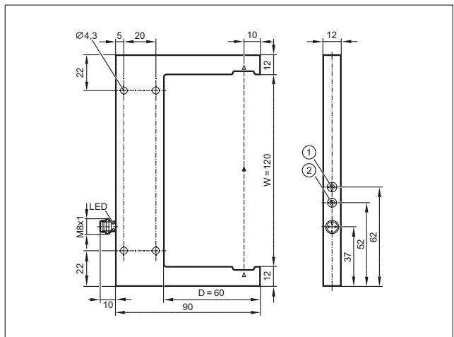
1: potentiometer sensitivity, 2: output function switch
