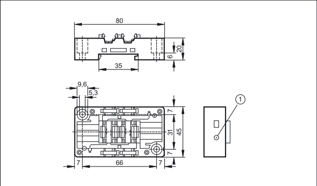
1: Addressing socket
