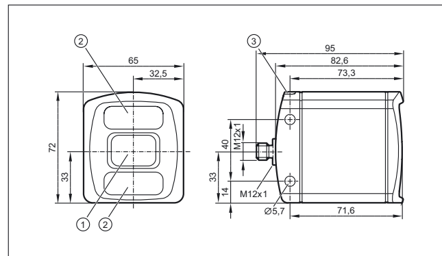
1: lens, 2: Illumination unit, 3: LED 2 colours (yellow/green)
