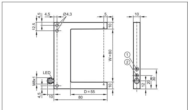
1: potentiometer sensitivity, 2: output function switch
